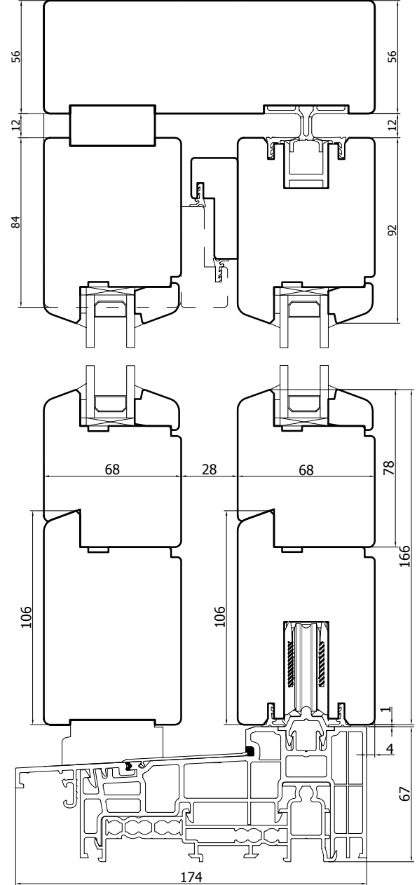
PRÓG HS G-U THERMOSTEP
