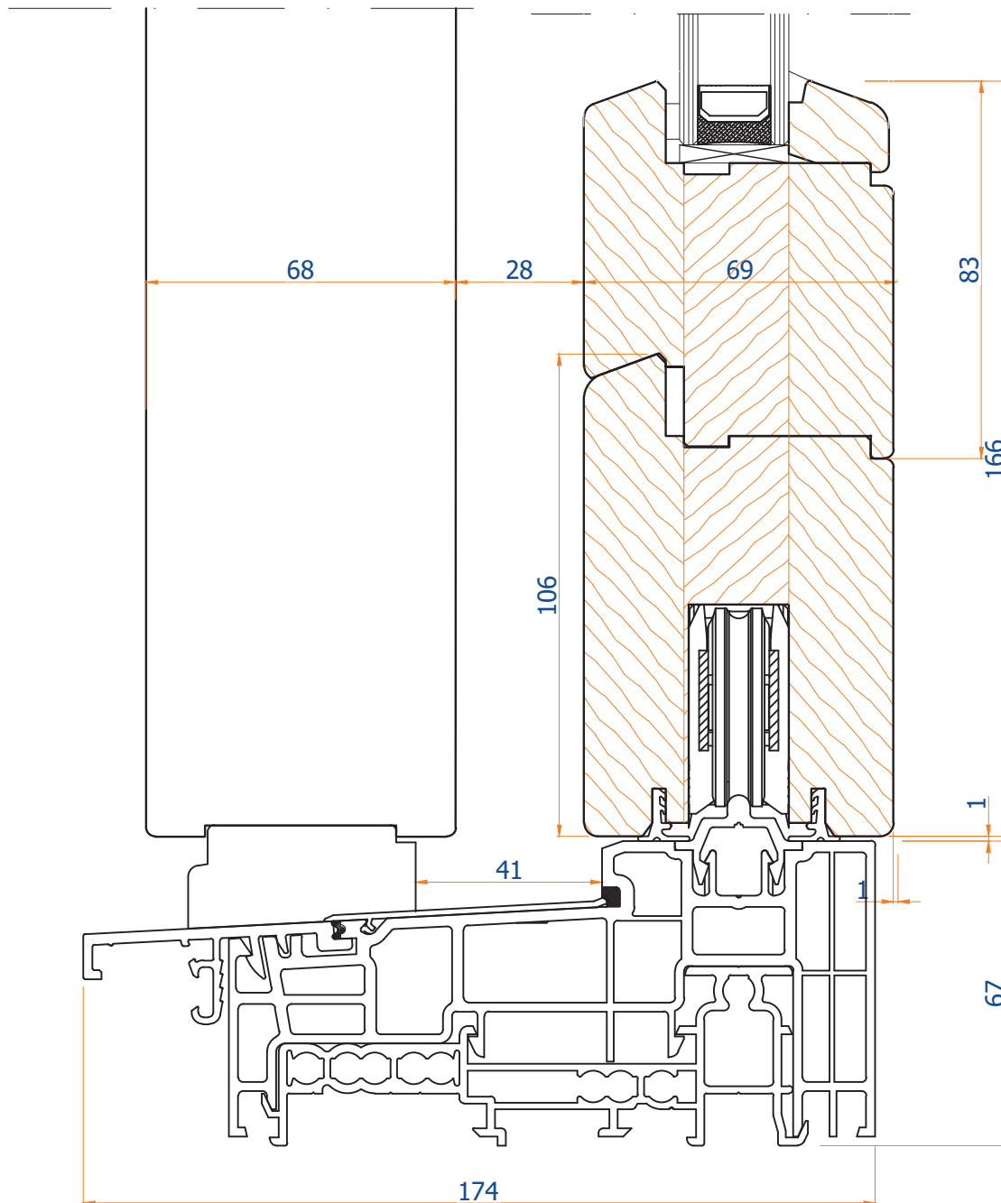
PRÓG HS G-U THERMOSTEP
